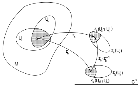
Figure 1: Coordinate maps on complex manifolds
