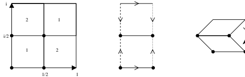
Figure 4: T^2/\mathbb{Z}_2
