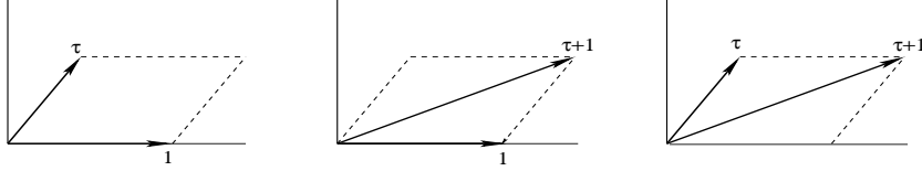
Figure 5: Three equivalent T^2 lattices
