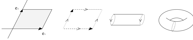
Figure 2: T^2 = \mathbb{R}^2/\Lambda
