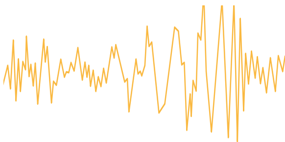
Figure 1. The first gravitational wave ever detected.
