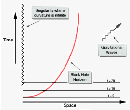
geodesic slicing \alpha = 1
