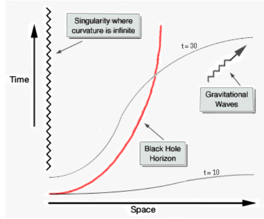
maximal slicing K = 0 \rightarrow -\nabla^i \nabla_i \alpha + \alpha(\tilde{A}_{ij} \tilde{A}^{ij} + \frac{1}{3} K^2) + \mathcal{L}_\beta K
